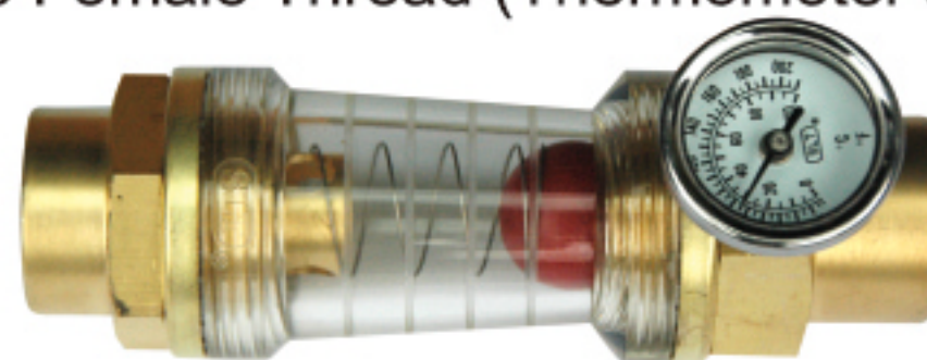
ST-04TA 雙內牙 ▼ 1/2"PT ~ 1"PT Double Female Thread
